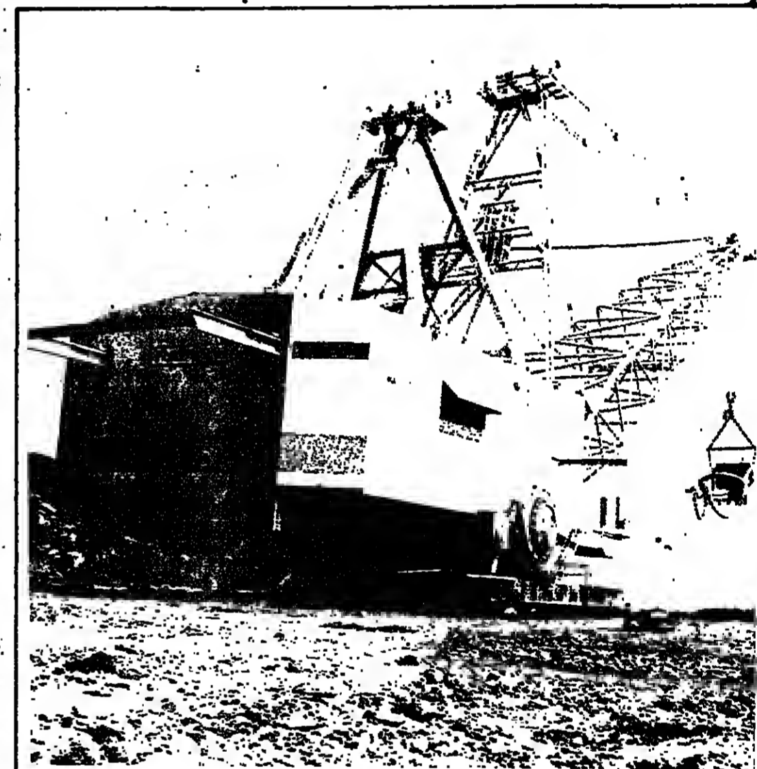
A Ransomes and Rapier walking dragline of the same type purchased by the Jordan Phosphate
